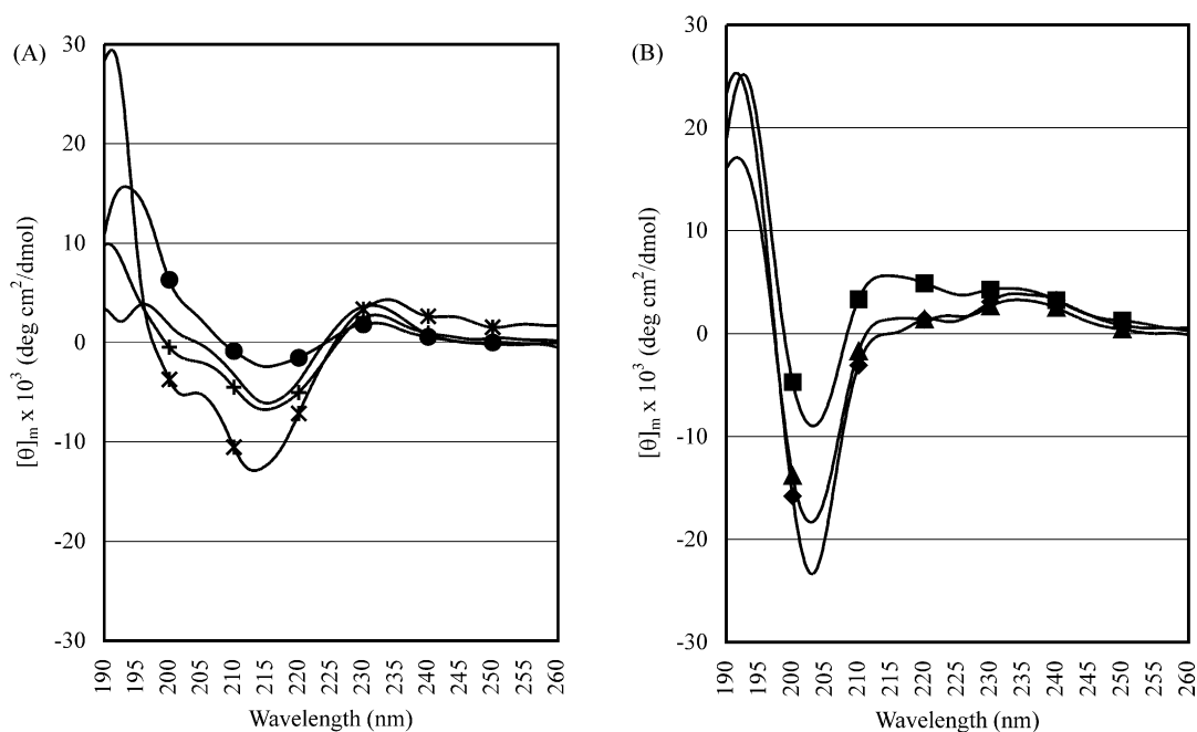
Figure 3. (A) CD spectra of EM-2 and its analogues in neat TFE. 1.31 mM EM-2 (1) (—), 1.47 mM Tyr-Pro-Phe-NH 2 (2) (●), 0.81 mM Tyr-Pro-Phe-NH-Phenethyl (4) (+), and 1.24 mM Tyr-Pro-Phe-Ala-NH 2 (8) (*). (B) 1.0 mM [Dmt 1 ]EM-2 (9) (▲), 1.45 mM Dmt-Pro-Phe-NH 2 (10) (■) and 0.79 mM Dmt-Pro-Phe-NH-Phenethyl (12) (◆).
