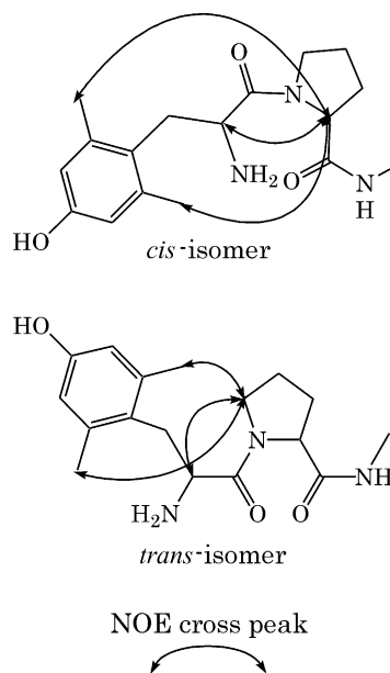
Figure 2. Characteristic NOE pairs of cis/trans configuration at the Dmt 1 -Pro 2 peptide bond.
