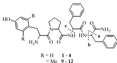
Figure 1. Structures of endomorphin 2 analogues.
